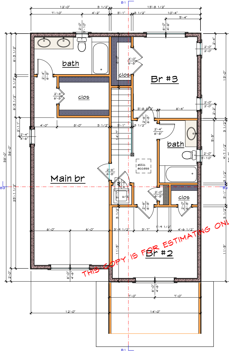
Floor 2 plan scale 1/4"=1'-0"
